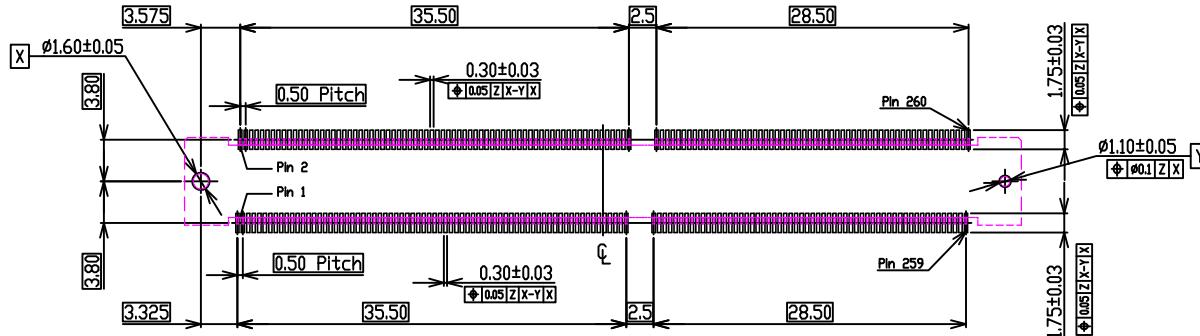
RECOMMENDED P.C.B LAYOUT ( \pm 0.05 )
