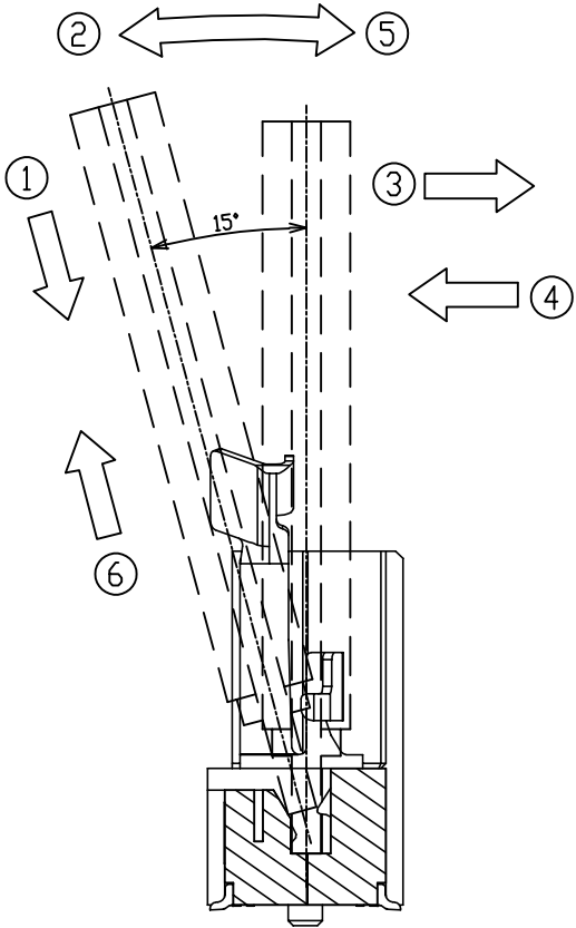
How to Mate And Unmated (SCALE 2:1)
