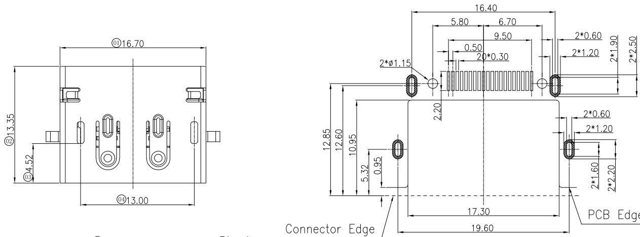
RECOMMENDED PCB LAYOUT (THICKNESS=1.20±0.05mm)
